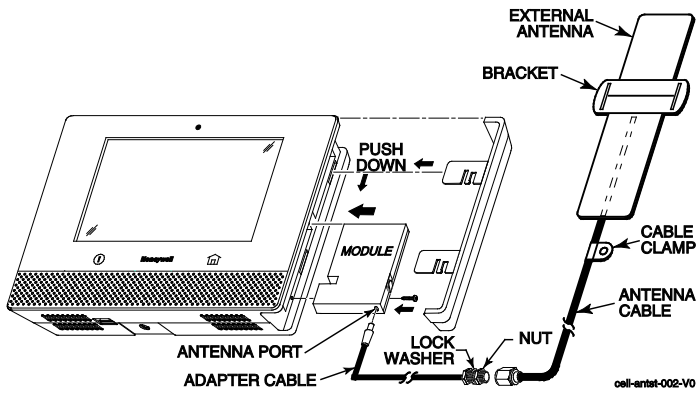
Connecting an External Antenna
